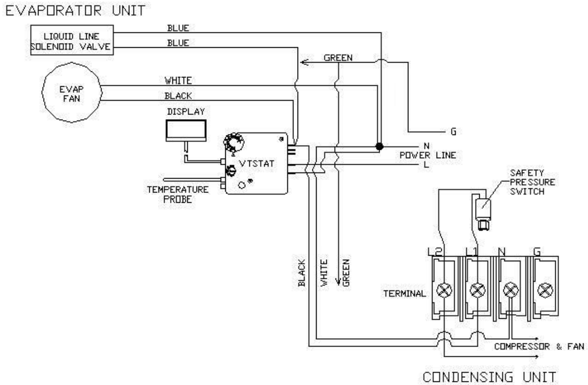
Fig. 2.2 VINO1500-4500SSL Electrical Wiring Diagram (VTSTAT)
