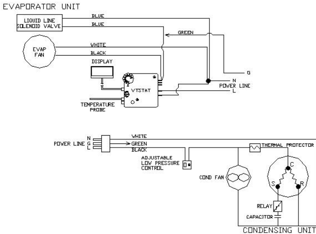
Fig. 2.4 VINO6500SSL Electrical Wiring Diagram (VTSTAT)
