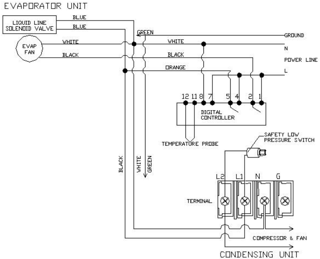
Fig. 2.3 VINO1500-4500SSL Wiring Diagram (DIGITAL CONTROLLER)
