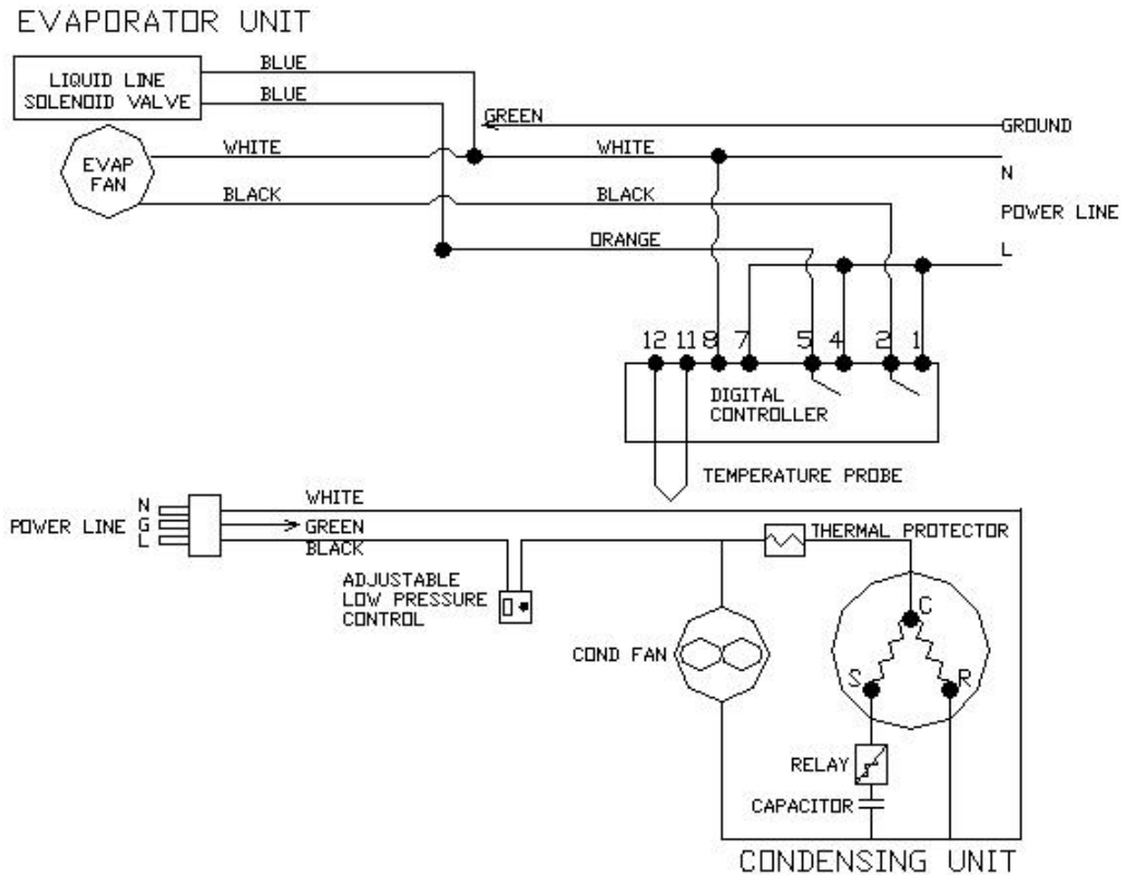
Fig. 2.5 VINO6500SSL Electrical Wiring Diagram (DIGITAL CONTROLLER)
